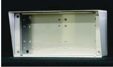
stainless steel enclosure model: ENCSSH height: 133.0mm width: 275.0mm depth: 85.0mm
